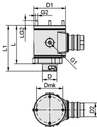
Design data VEE-RU 55x83.5 60 QCM
