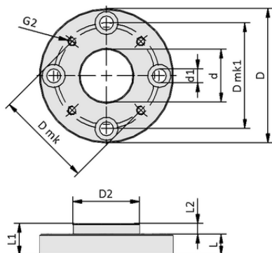
Design data FLAN-PL 63.5x10 AL-EL VEE
