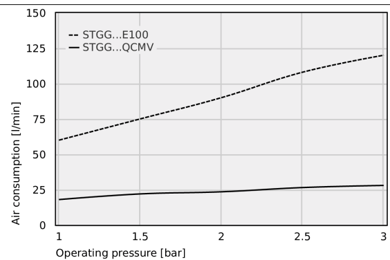
Air consumption
