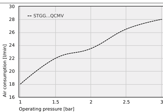
Air consumption
