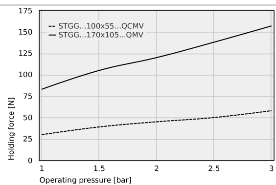
Holding force
