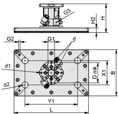
Design data STGG S 170x105 1xE100 A PEEK
