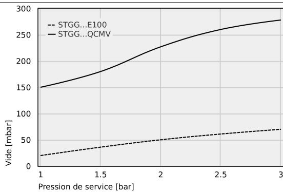
Vide ex cutable   diff rentes pressions de service
