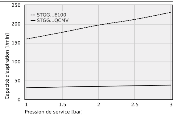
Capacit  d'aspiration   diff rents degr s d' vacuation
