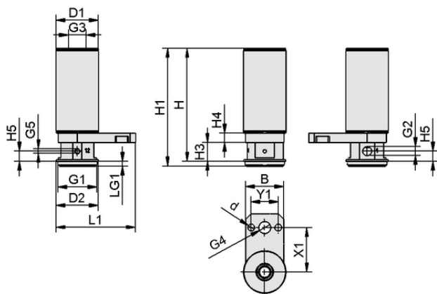
Design data SCG 1xE100 A MS SDA M37x1-AG
