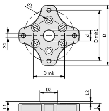
Design data FLAN-PL 55x7.5-EL1
