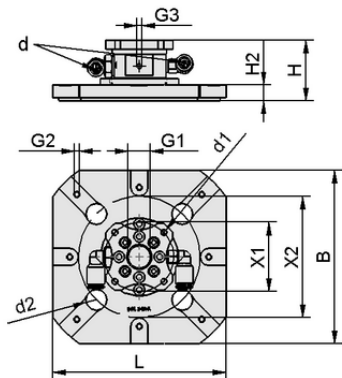
Design data SWGm-6A 146x146x40 1xE100 A PEEK
