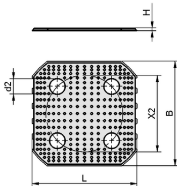
Design data SAUG-FL SWGm-6 141x141 PEEK
