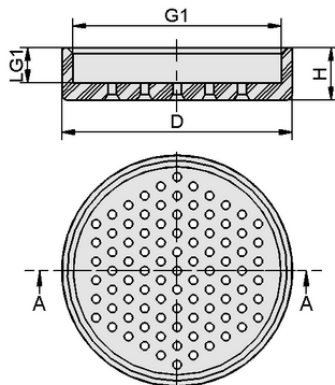
Design data SAUG-FL SCG 60 POM
