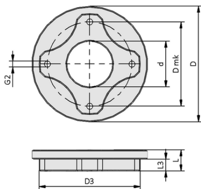
Design data FLAN-PL 63x11.5-UNI
