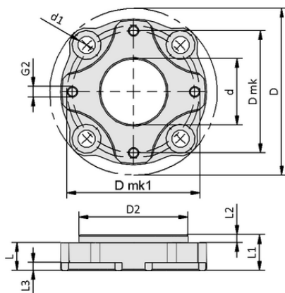
Design data FLAN-PL 63x10.5-AD1
