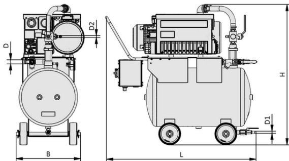
Design data VAGG 63 AC3 80 MD
