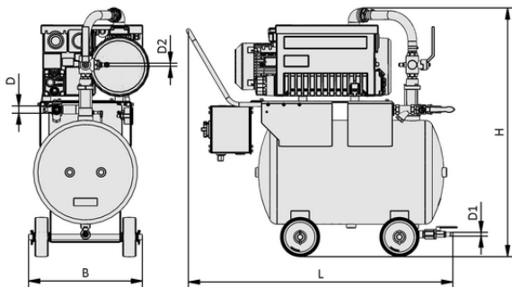
Design data VAGG 40 AC3 80 MD
