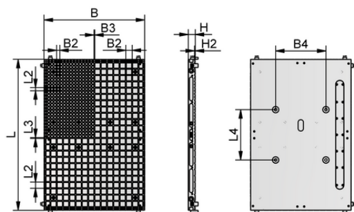
Design data MPL 300x200x28 12,5x12,5 3x3
