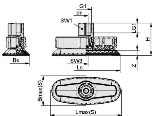
Design data SAOXM 80x30 ED-85 NPT3/8-IG
