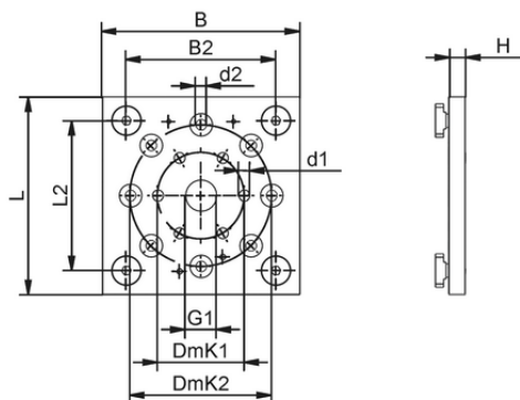
Design data SET FXC-FMC
