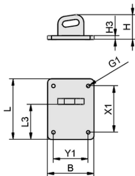
Design data MOD-FLAN 157x120 SBX-C
