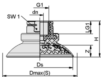
Design data SAX 80 ED-85 NPT3/8-IG
