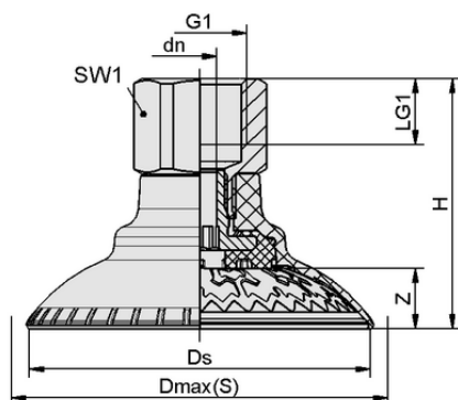
Design data SAXM 60 ED-85 NPT3/8-IG
