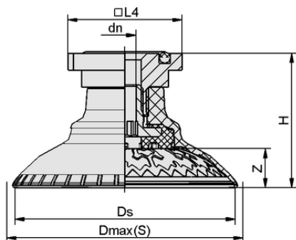
Design data SAXM 80 ED-85 RA
