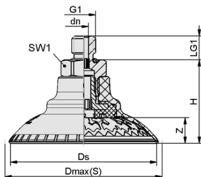
Design data SAXM 60 ED-85 M14x1.5-AG
