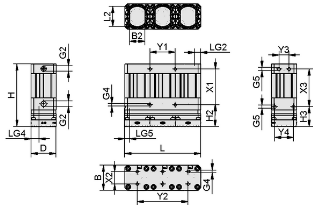
Design data SGM-HT-HP 40x121 3RR
