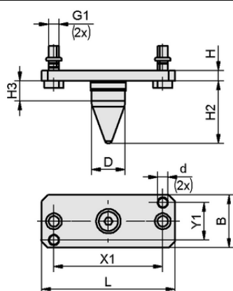
Design data GR-E SGM-HPm 40 CP9.6 SET
