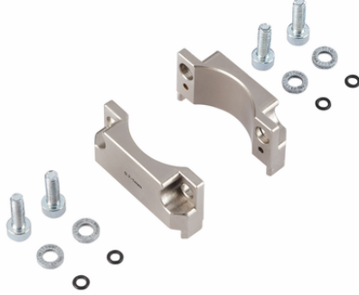
GR-E SGM-HPm 40 DES 0.7 SET
