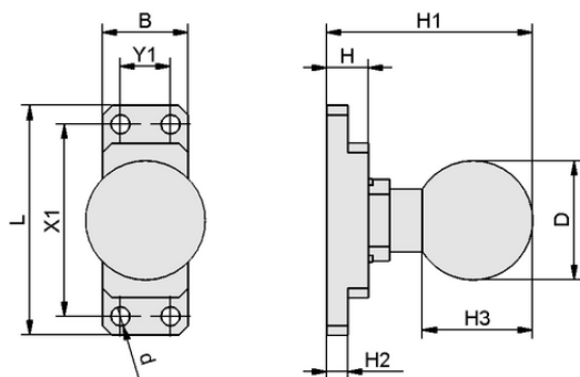
Design data HTS-A5 SGM-HP 20 OP
