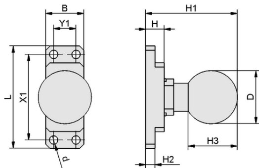
Design data HTS-A3 SGM 50/70 OP
