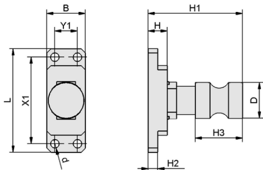
Design data HTS-A2 SGM-HP 50 OP
