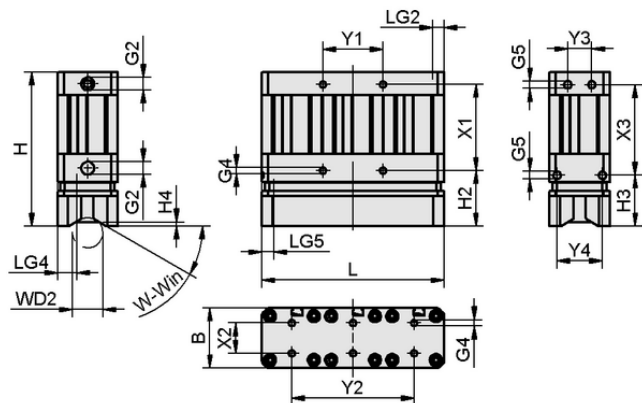
Design data SGM-HP 40x121
