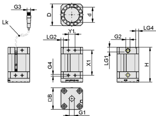
Design data SGM-HD-S 30 G1/8-IG PNP
