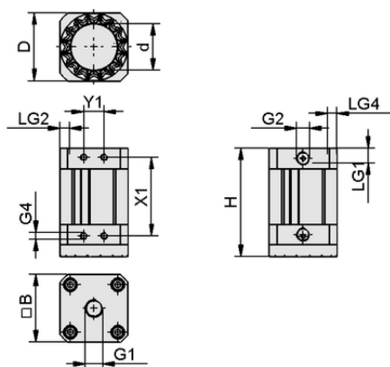
Design data SGM 50 G1/4-IG
