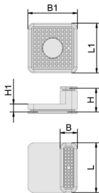
Design data ISBL-HD 80x28x38
