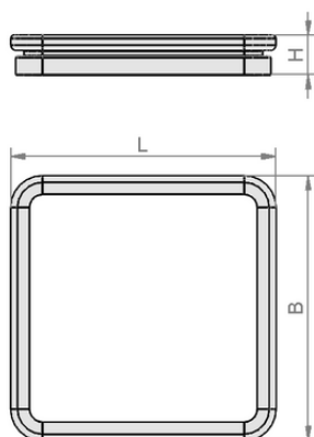
Design data ISDR 100x100x12 Cup 4
