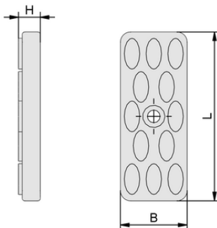
Design data ISRPL 66x66x8.5 NK-45 d12
