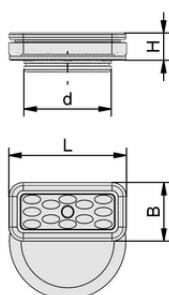
Design data ISCUP Cup 2 80x40x16
