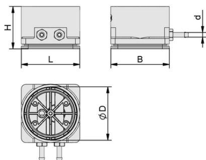
Design data ISMB-G 80x80x70
