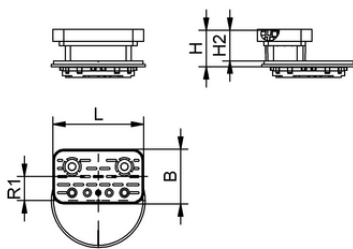
Design data VCBL-S6-CUP 125x75x85 TV+ME
