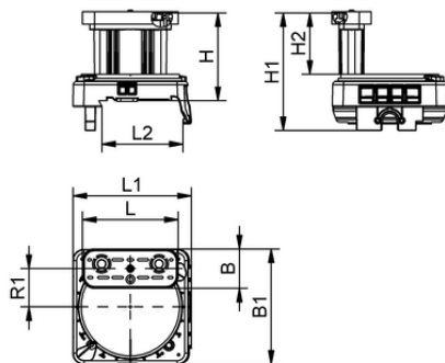
Design data VCBL-S6 130x30x50 S-360-15 TV
