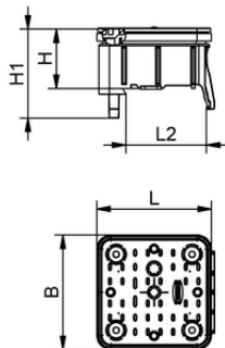
Design data VCBL-S6 145x145x50 TV+ME
