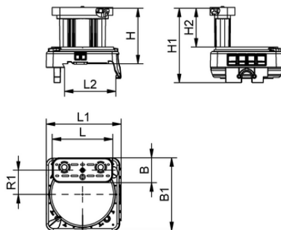
Design data VCBL-S6 130x30x75 S-360-15 TV
