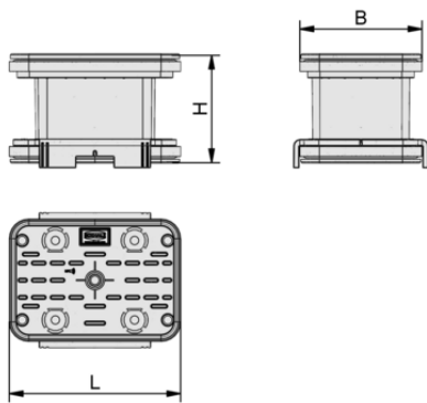
Design data VCBL-K2-PRO 160x115x100 TV
