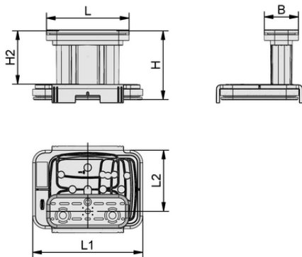
Design data VCBL-K2-PRO 130x30x100 L
