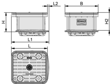
Design data VCBL-B 140x130x48 TV
