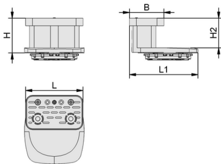
Design data VCBL-B 120x50x29 TV
