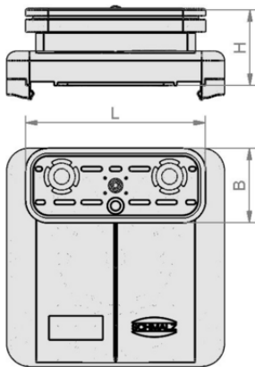
Design data VCBL-S1 120x120x50 TV
