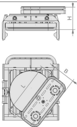
Design data VCBL-K1 130x30x125 D-360
