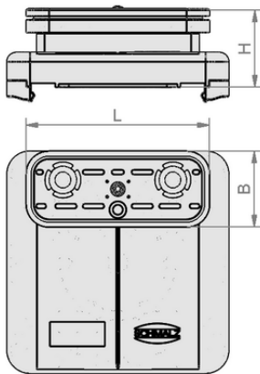
Design data VCBL-S1 130x30x32.7 TV-S
