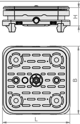
Design data VCBL-S1 120x120x32.7 TV-S
