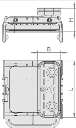
Design data VCBL-K1 125x75x125 L
