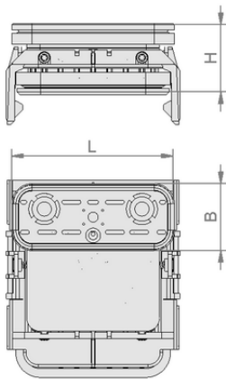
Design data VCBL-K1 125x75x125 Q
